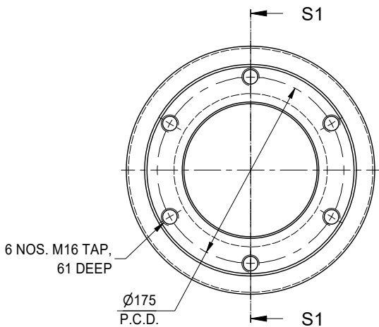
ELEVATION SCALE 1 : 5
