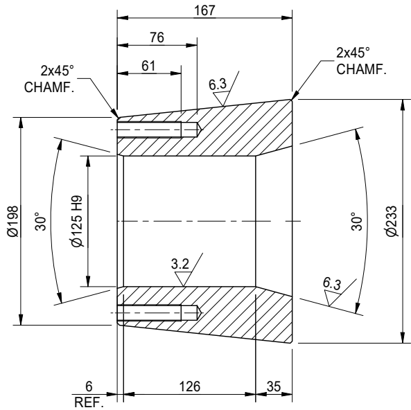
SECTION AT S1-S1 SCALE 1 : 5
